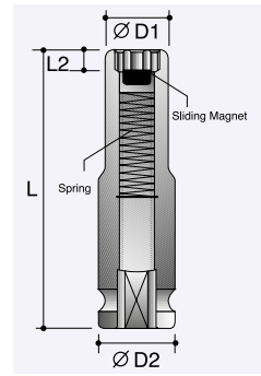
External Torx Sockets - Deep - With Slide Magnetic
