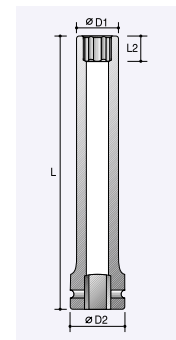
6-Point Extra Long Socket For Wheel Nuts
