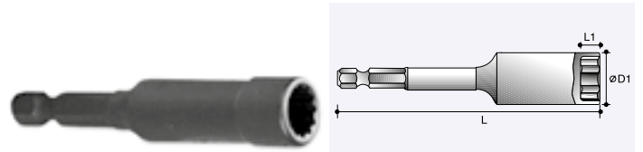
12-Point Sockets
