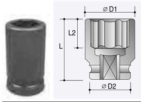
6-Point Budd Wheel Sockets - Control Depth Hex
