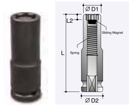
6-Point Sockets - Deep - With Slide Magnetic
