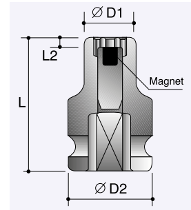
6-Point Sockets - With Magnetic
