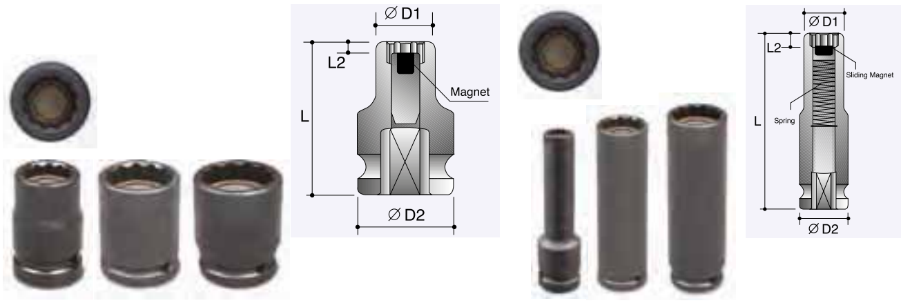
12-Point Sockets
