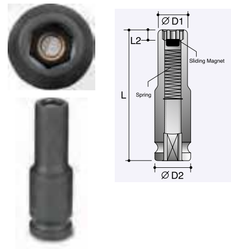
6-Point Sockets - Deep
