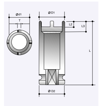
"GU" Type Axial Nut Sockets
