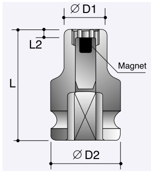
External Torx Sockets - With Magnetic
