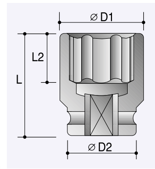
6-Point, Spindle Nut Impact Sockets
