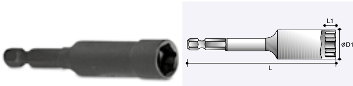
6-Point Sockets
